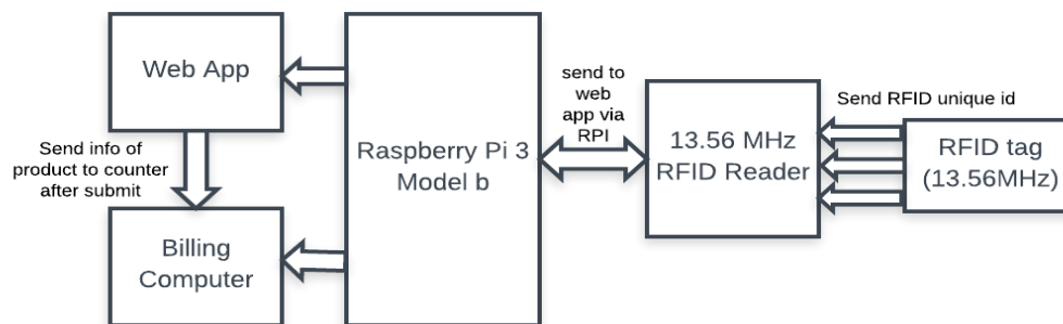
Figure 2: Block Diagram of Interfacing Units
