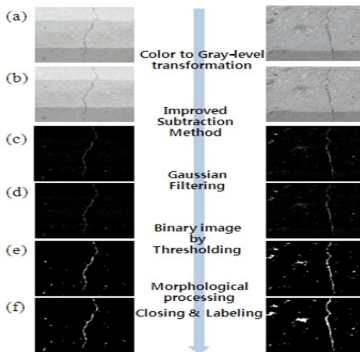
Figure 6: Result of the Proposed Image Processing
