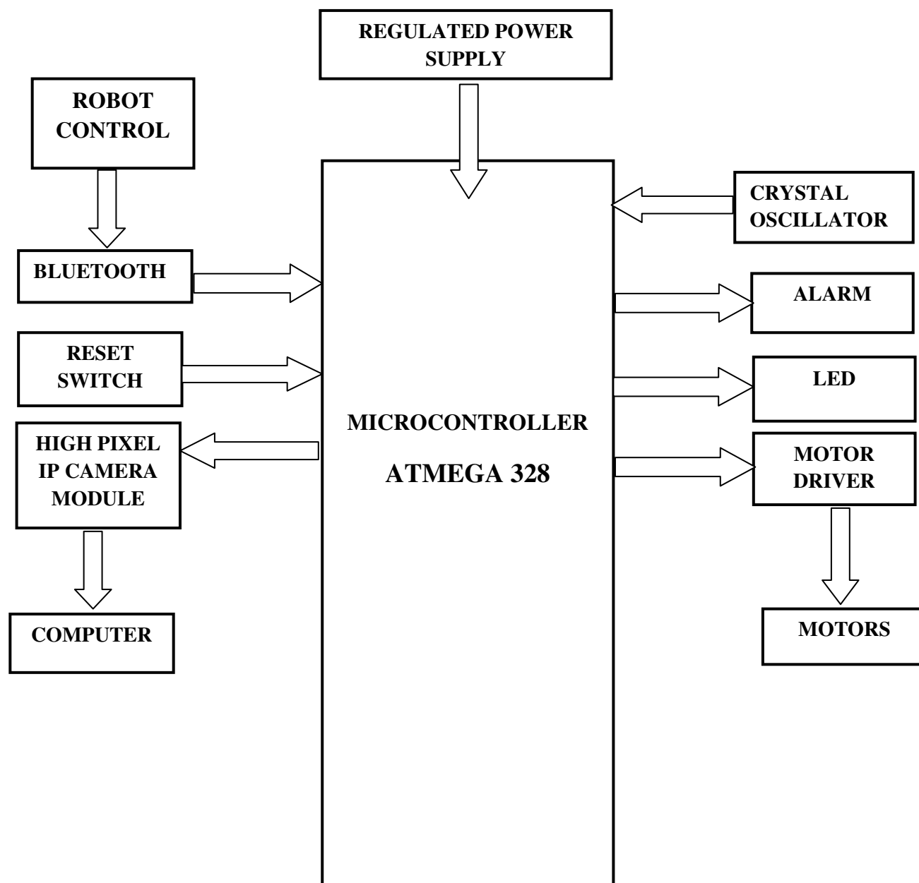
Figure 2: Block Diagram of Proposed System
