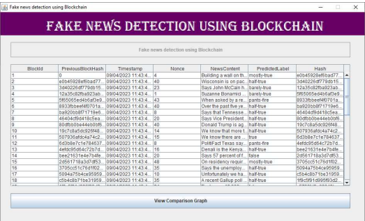
Figure 5. Blockchain
