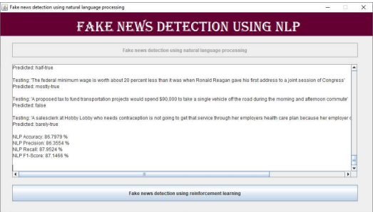
Figure 4. NLP
