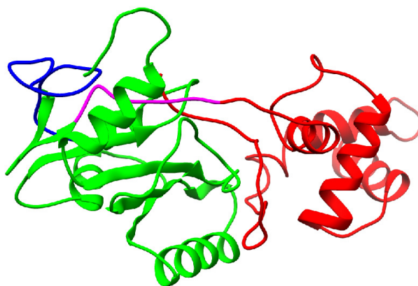
Fig. 1. Cartoon representation of RbgA. N-terminal domain represented by green color, C-terminal by red, switch-I and switch-II are highlighted with blue and magenta colors.
