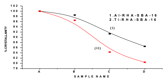
Fig8 : Effect of the metal concentration on PercentCrystallinity of RHA-SBA-16
