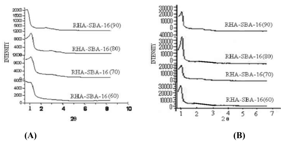
Fig. 1: XRD patterns of (A) as-synthesized and (B) calcined samples of RHA-SBA-16(60°C to 90°C) for synthesis temperatures 60 0 -90 0 C
