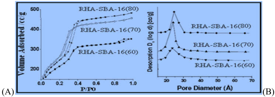
Fig.3: (A) N 2 adsorption-desorption isotherms and (B) pore size distribution of RHA-SBA-16 (60, 70, 80) synthesized at 60 0 -80 0 C
