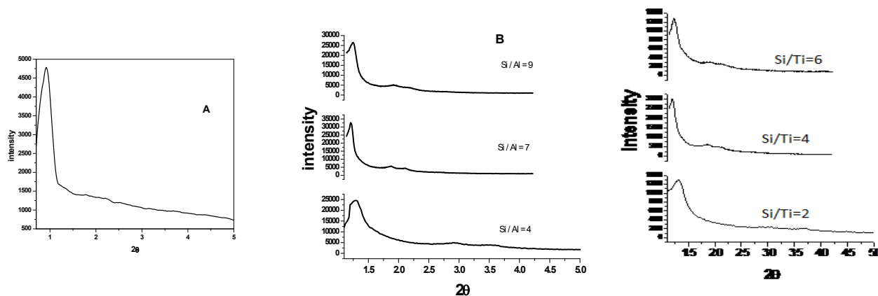
Fig. 7 : A) XRD patterns of calcined parent RHA-SBA-16 sample.
