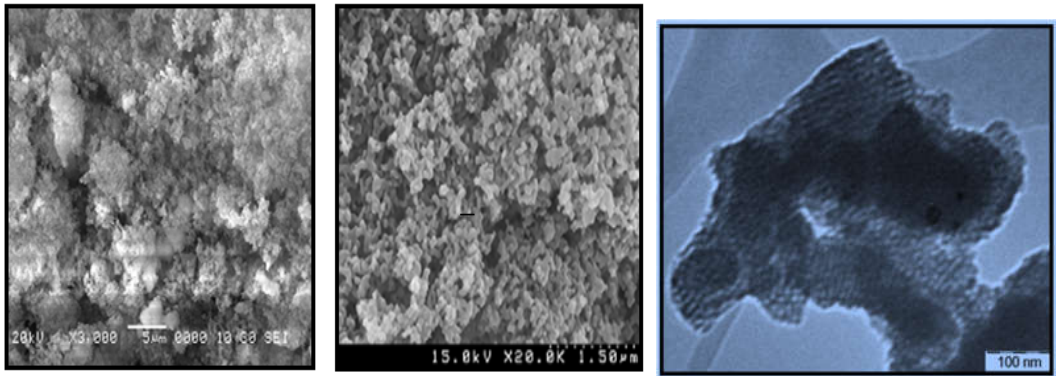
Fig. 4: SEM images of RHA-SBA-16(60, 80) synthesized at 60 and 80 0 C Fig. 5: TEM images of RHA-SBA-16(80) synthesized at 80 0 C
