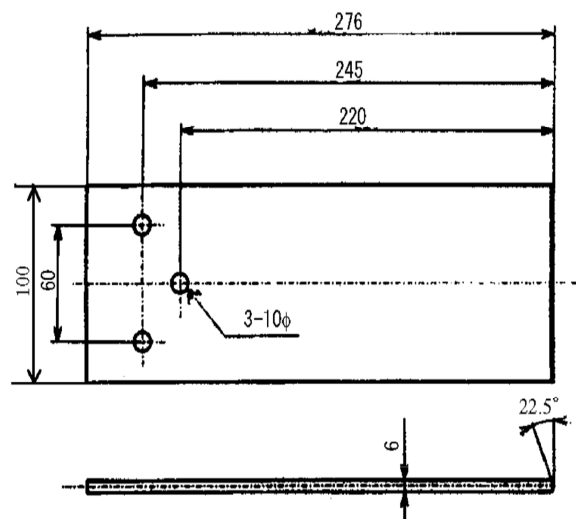
Fig.1 Geometry of the model used in the Analysis
