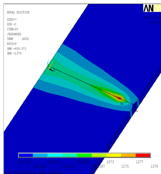
Fig.2 TEMPERATURE DISTRIBUTION AFTER WELDING
