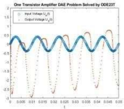
Fig. 4.2 Output of ODE23T DAE solution
